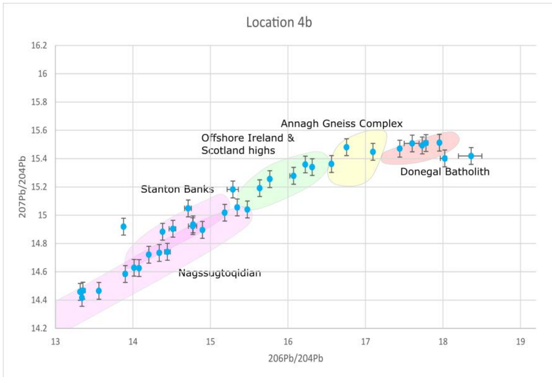
SD5: Pb isotopic ratios of K-feldspar for individual locations. Error bars are indicated on data points. Potential source domains are represented as coloured polygons.
