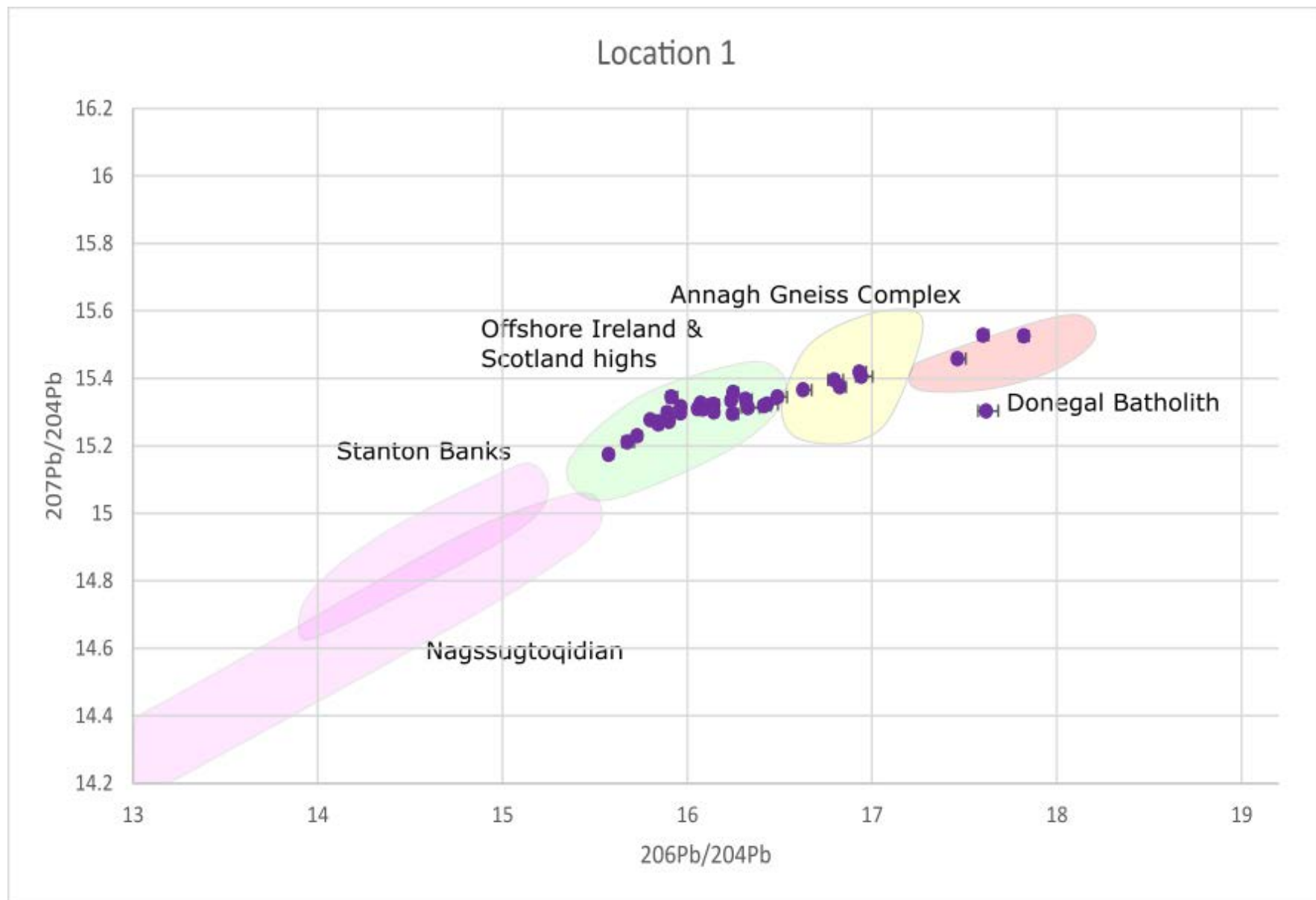
SD1: Pb isotopic ratios of K-feldspar for individual locations. Error bars are indicated on data points. Potential source domains are represented as coloured polygons.
