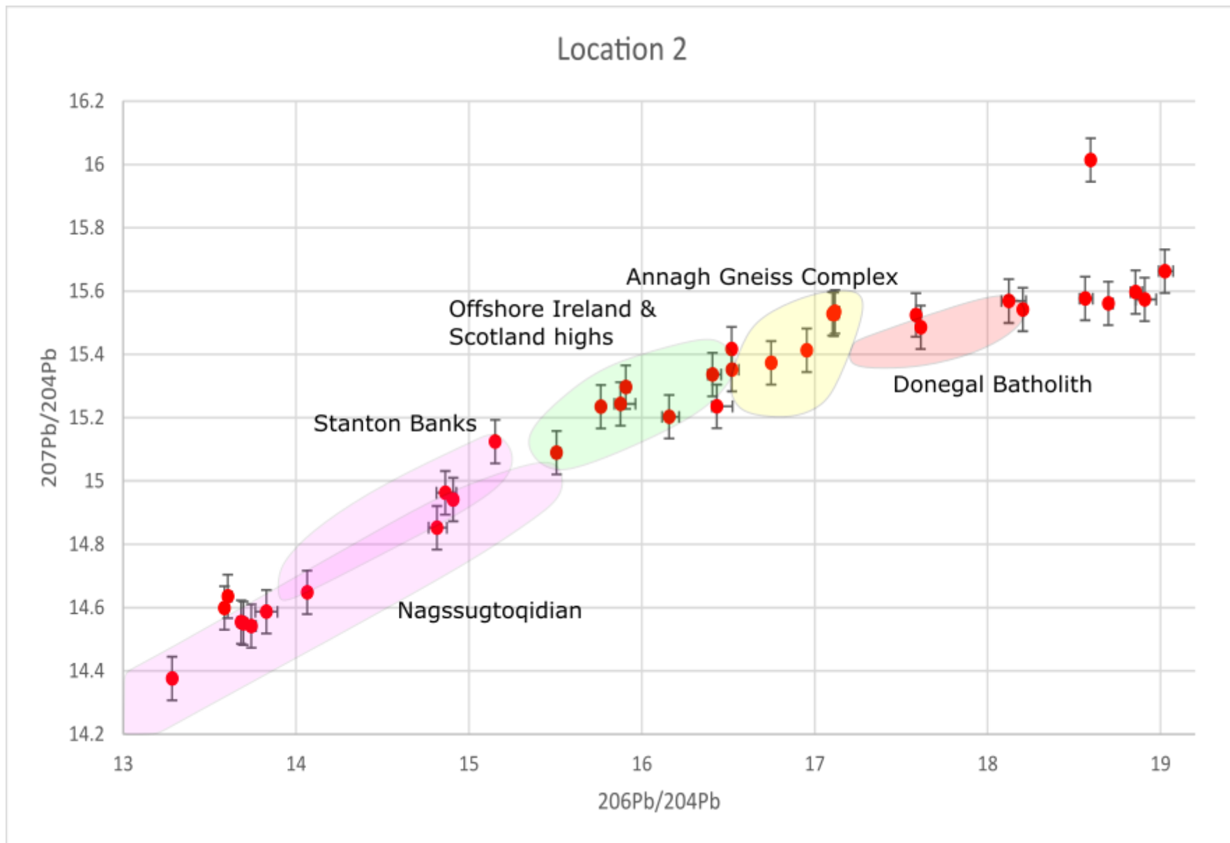
SD2: Pb isotopic ratios of K-feldspar for individual locations. Error bars are indicated on data points. Potential source domains are represented as coloured polygons.
