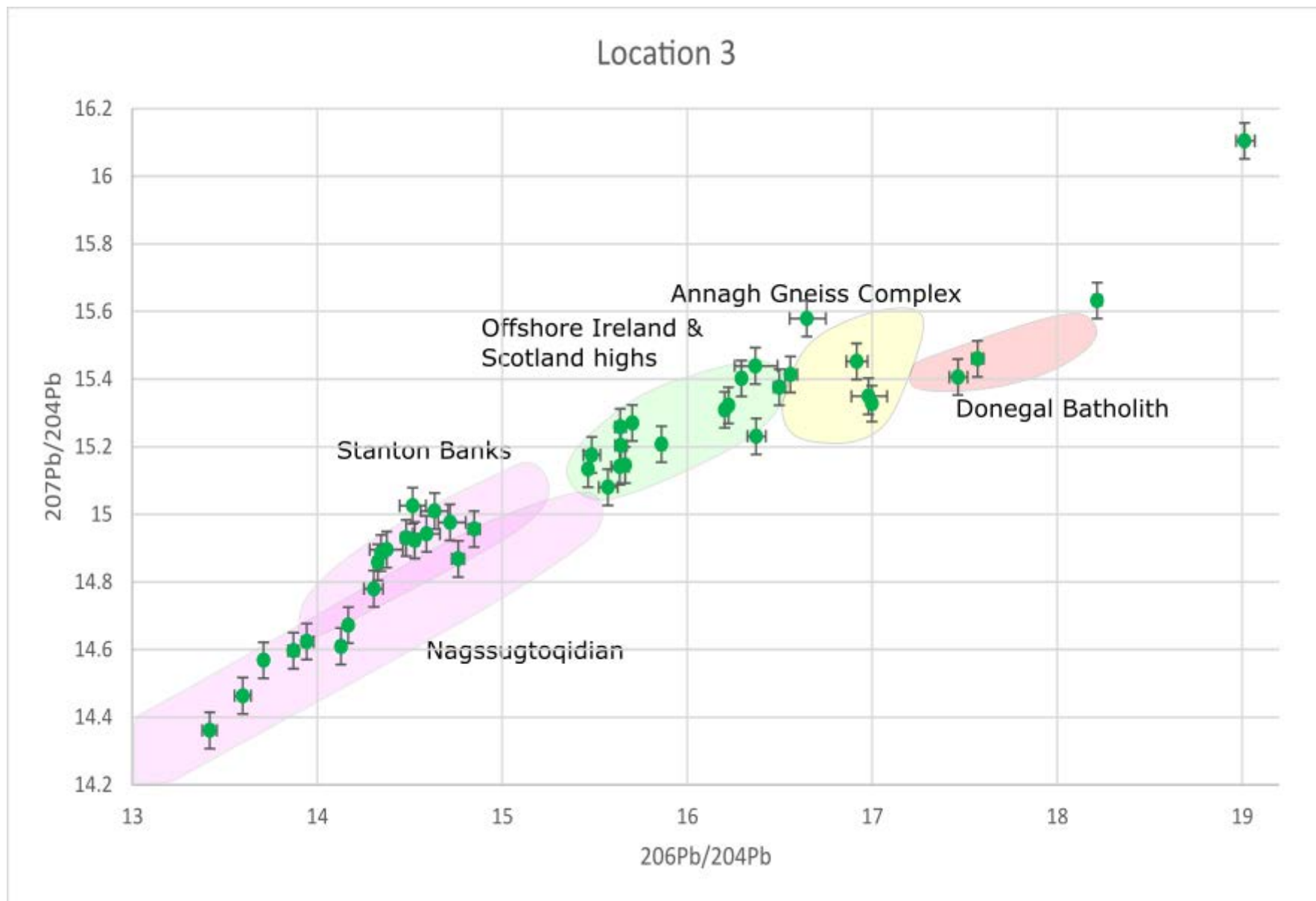
SD3: Pb isotopic ratios of K-feldspar for individual locations. Error bars are indicated on data points. Potential source domains are represented as coloured polygons.
