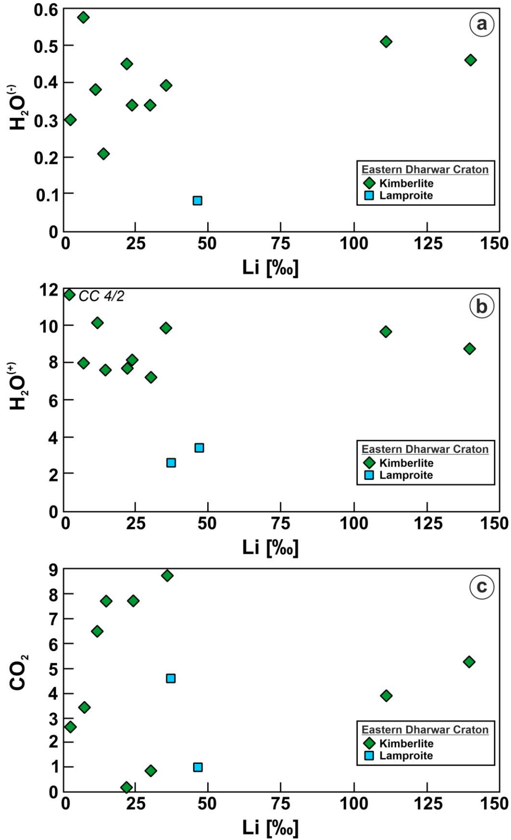
Fig. S1. Li v. H_2O^{(-)} (a), Li v. H_2O^{(+)} (b) and Li v. CO_2 (c) diagram for studied kimberlites and lamproites from the Eastern Dharwar Craton.
