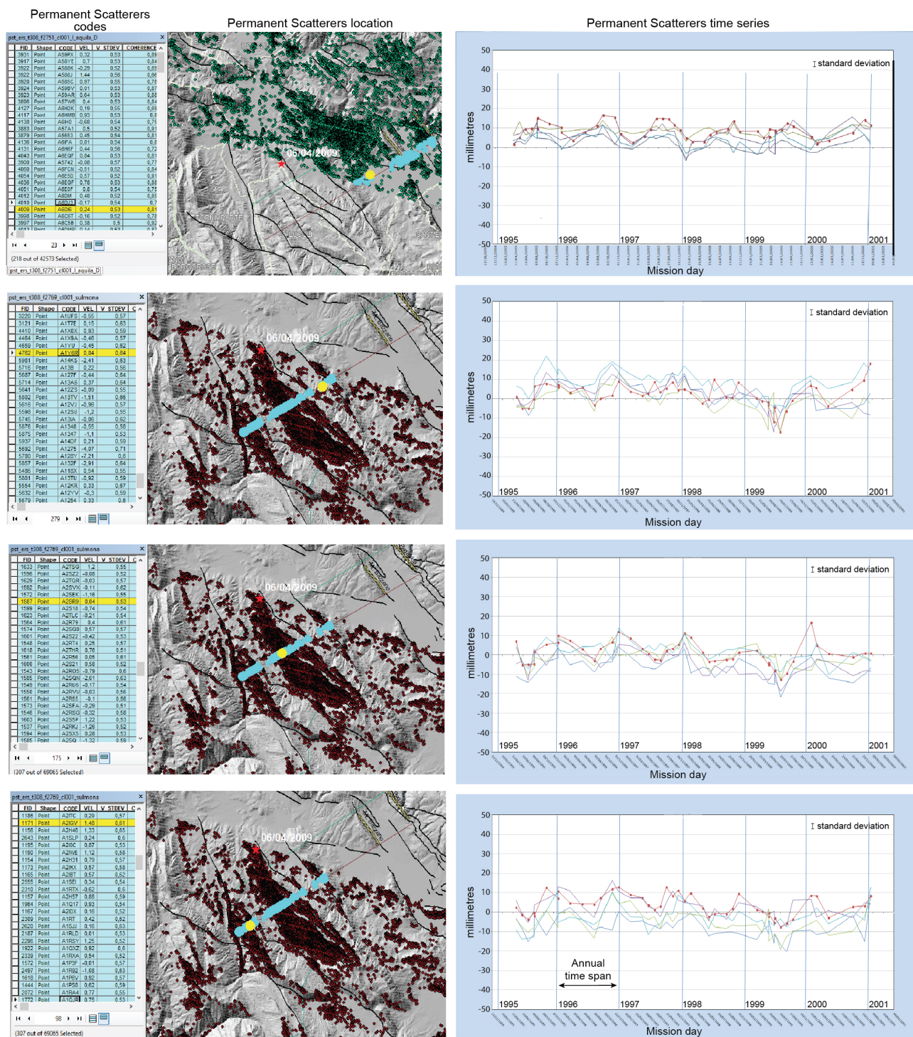
Figure S2. Examples of raw time series of Permanent Scatterers obtained from ERS descending orbit images. The column in the right side shows time series of groups of closely spaced PS, with indication of correlative locations (yellow dots in images in the central column) and codes, shown in the table images reported in the column in the left side. The error bars represent standard deviation of the measurements.
