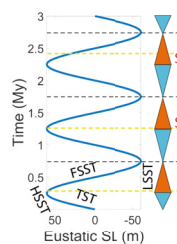
Model Run 62: eustatic control
