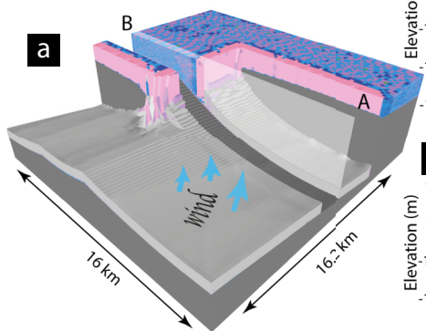
Model Run 61: base model
